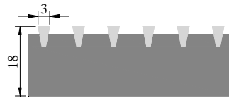
Cross-section of stainless steel grille
