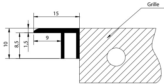
Frame type F
