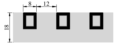
Cross-section of linear grille painted in RAL
