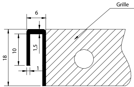
Frame type L
