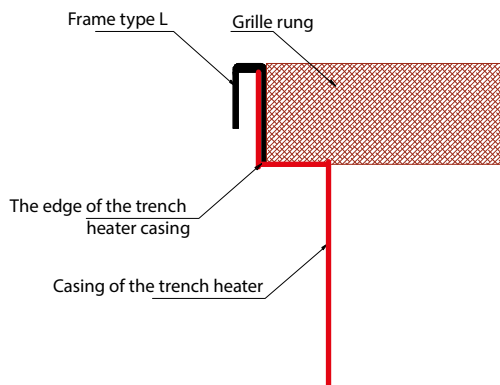
Frame type L
